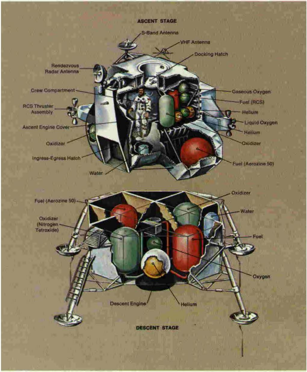
Diagram of the Lunar Module spacecraft.
